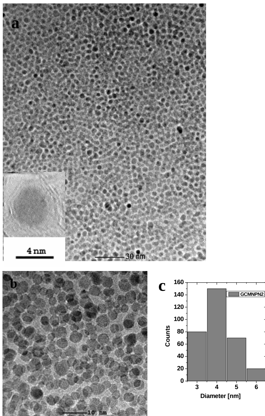
Figure VIII.2 TEM images (a, b) and nanoparticles size distribution histograms (c), of GCMNPN2. The inserts in the figure show a nanoparticle covered by 1-2 layers graphene
