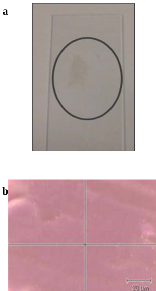
Figure VI.2 Photograph of graphene transferred on a glass slip (a) optical image of the transferred few layer graphene on SiO 2 /Si (b)
