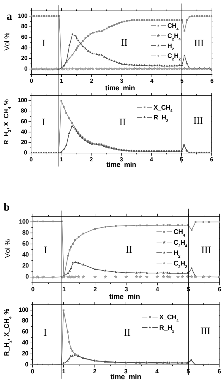
Figure VII.16. On line analysis and \text{CH}_4 conversion and \text{H}_2 yield during the test: for GCMNP3 synthesis (a); for GCMNP4 synthesis (b)
