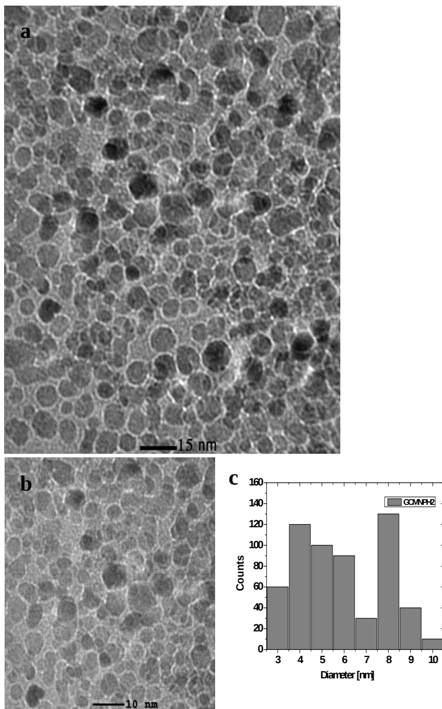
Figure VIII.1 TEM images (a, b) and nanoparticles size distribution histograms (c), of GCMNPH2
