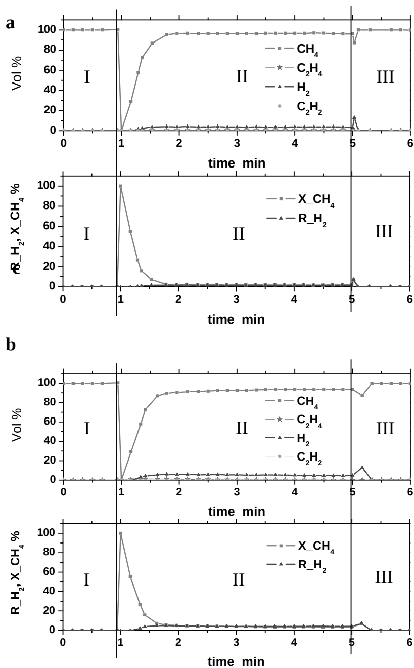
Figure VII.10 On line analysis and \text{CH}_4 conversion and \text{H}_2 yield during the test: for an empty reactor (a); and in presence of non impregnated gibbsite, treated as GCMNP2 (Al2 in Table VII.2)(b)
