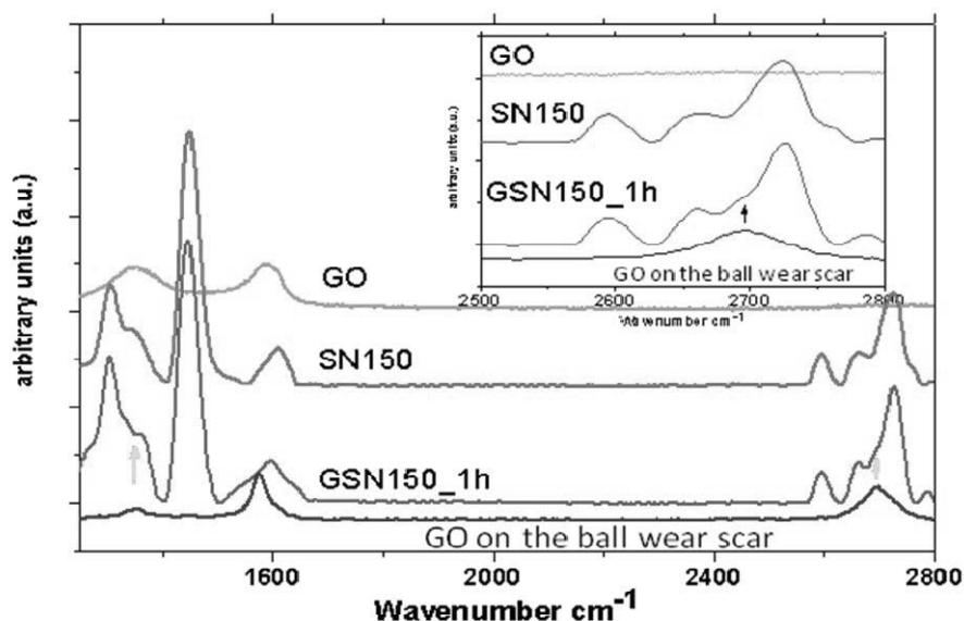
Figure IX.10 Raman spectra of GO, SN150, GSN150_1h and GO on the ball wear scar after 1 hour test at p=1.68\text{ GPa} , T=25\text{ }^{\circ}\text{C} , v=0.5\text{ m/s}
