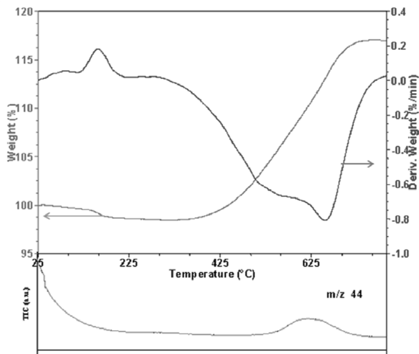
Figure VII.6 TG-DTG_MS analysis of GCMNP1 after alumina removal
