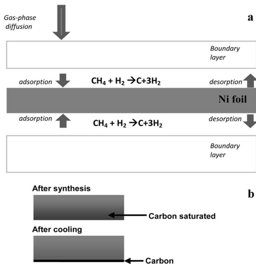
Figure V.13 Reaction synthesis scheme (a). Nickel saturated by carbon after synthesis, and the carbon layer covering the bottom Ni surface at the end of cooling (b)
