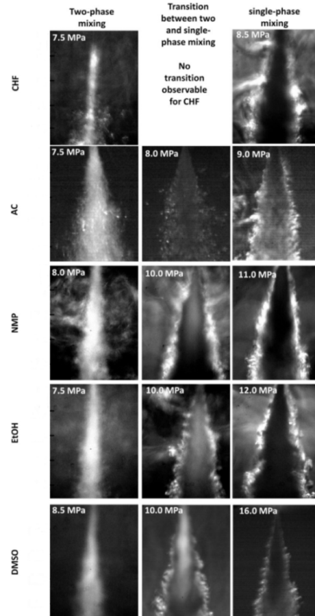
Figure II. 5 Jet images of CHF, AC, NMP, EtOH and DMSO injected at 313 K with a flow rate of 2.5 mL/min through the \varnothing = 80 \mu\text{m} nozzle into \text{scCO}_2 (from (De Marco et al., 2012)).
