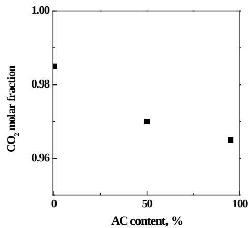
Figure IV. 10 CO 2 molar fraction ( X_{\text{CO}_2} ) varying the AC content in the mixture EtOH/AC.
