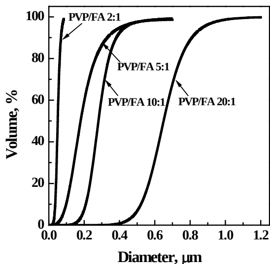
Figure V.4 Volumetric cumulative PSDs of PVP-FA nano and sub-microparticles precipitated from DMSO at 15.0 MPa and 313 K at different polymer/drug ratios.
