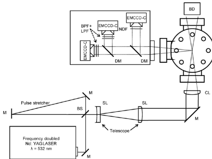
Figure IV. 5 Schematic of the experimental setup, (M: mirror, BS: beam splitter, SL: spherical lens, CL: cylindrical lens, BD: beam dump, DM: dichroitic mirror, NDF: neutral density filter, BPF: band pass filter, LPF: long pass filter, EMCCD-C: electron multiplying charge coupled device camera) (from (Dowy et al. , 2010)).
