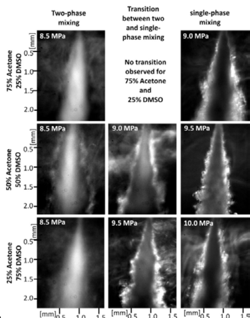
Figure IV. 2 Jet images of solvent mixtures of DMSO and AC injected at 313 K with a flow rate of 2.5 mL/min through a \varnothing = 80 \mu\text{m} nozzle into \text{scCO}_2 (De Marco et al., 2012).
