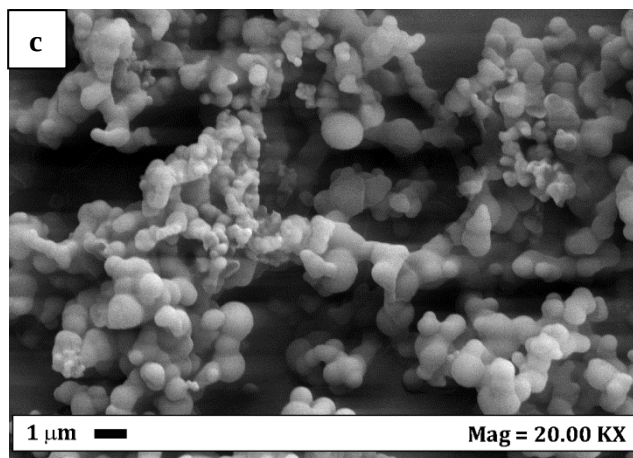
Figure IV.17 FESEM images of cellulose acetate precipitated at 9.0 MPa, 40°C, 60 mg/mL at different DMSO/Acetone mixtures percentages; (a) 25/75 (v/v); (b) 50/50 (v/v); (c) 75/25 (v/v).
